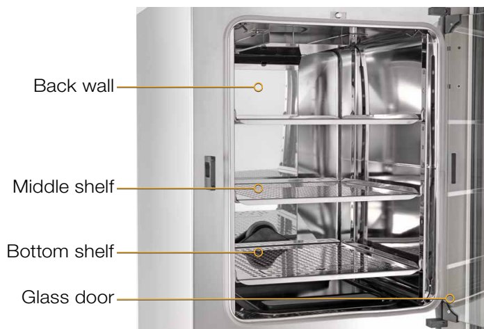
Figure 1. Interior of a Thermo Scientific CO 2 incubator with the Steri-Run cycle, indicating the locations of coupons containing test microorganisms.
