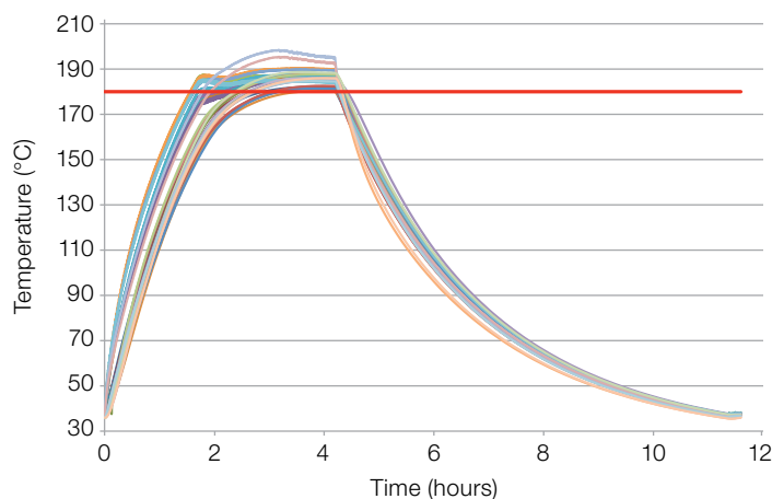
Figure 4. Typical temperature map for a full Steri-Run cycle. Thermocouples were placed in 48 locations in the chamber, including the walls, glass door, water reservoir cover and floor, and 3 shelves. All areas reached a minimum of 180°C. N = 2 x 4 units.
